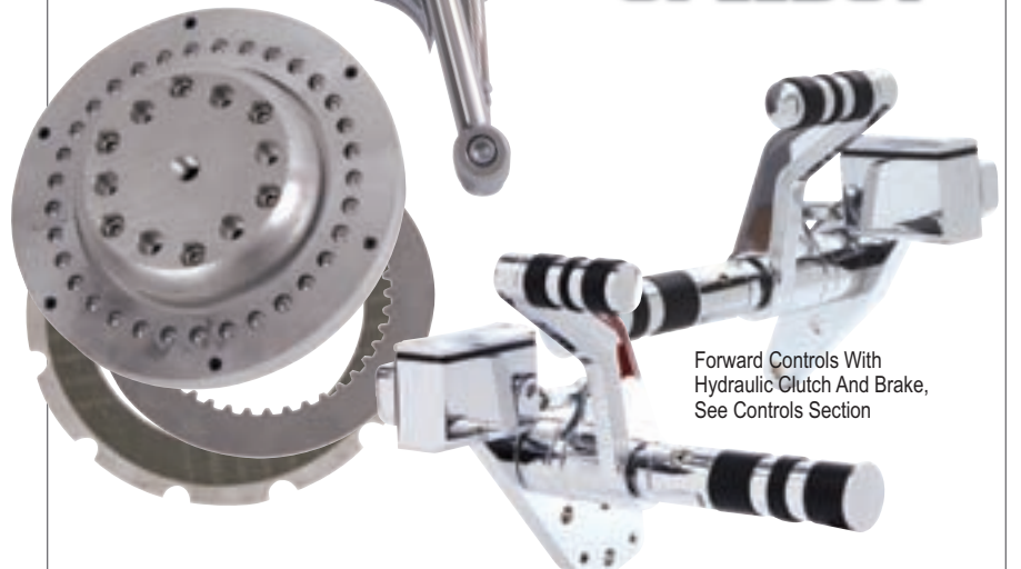
Auto Clutch For BDL, High-Tech & Primo®
